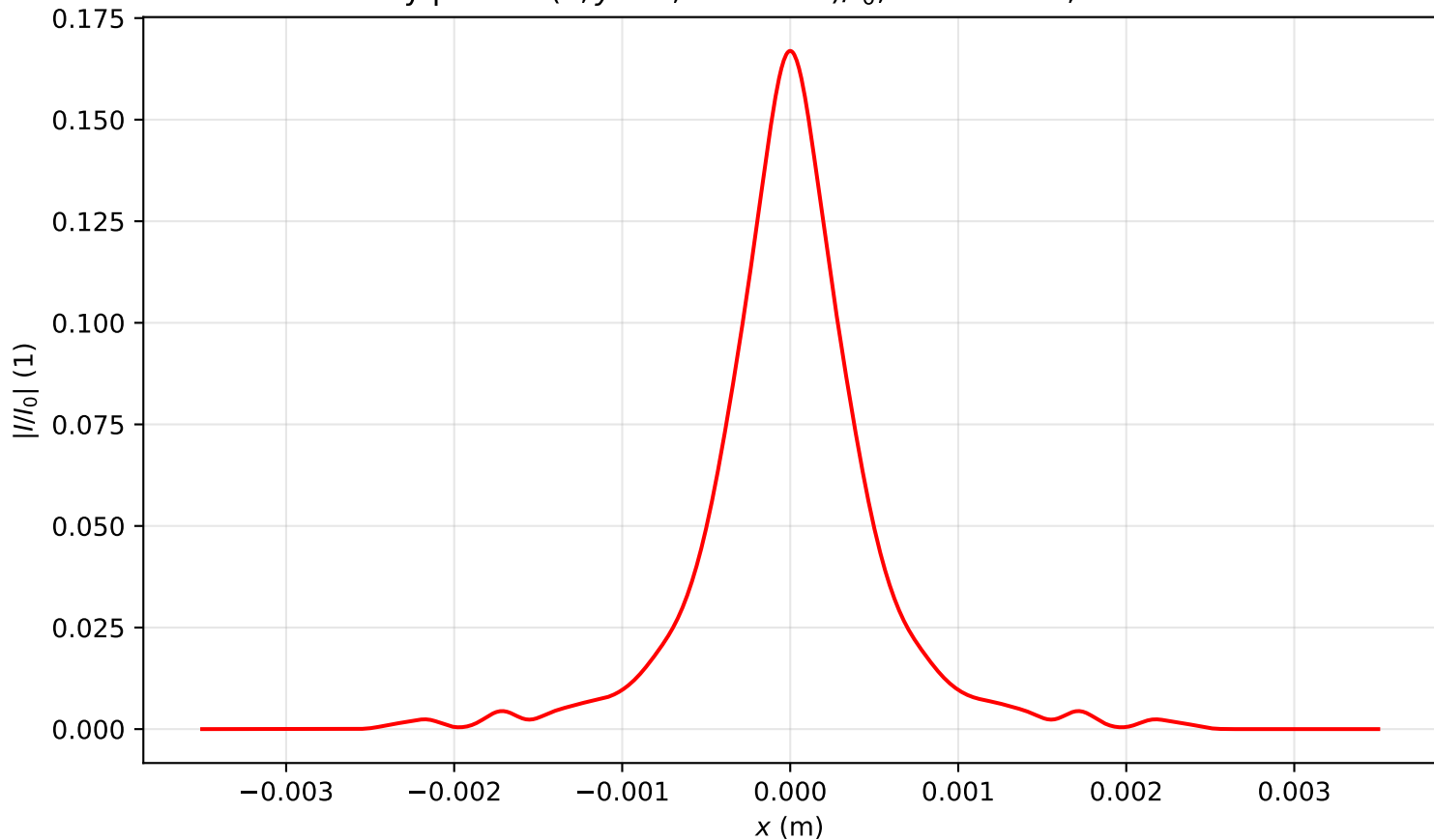
Intensity profile I(x, y = 0, z = 3.662)/I_0 , \text{Pin}=5.0\text{Pcr} , artificial time
